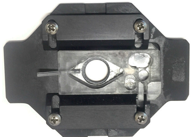
Fig. 2. This figure is a picture of the chamber used in the various experiments to image the changes in the shape (volume) of individual ghosts on changes in the tonicity of the medium, as detailed in the Materials and Methods .
